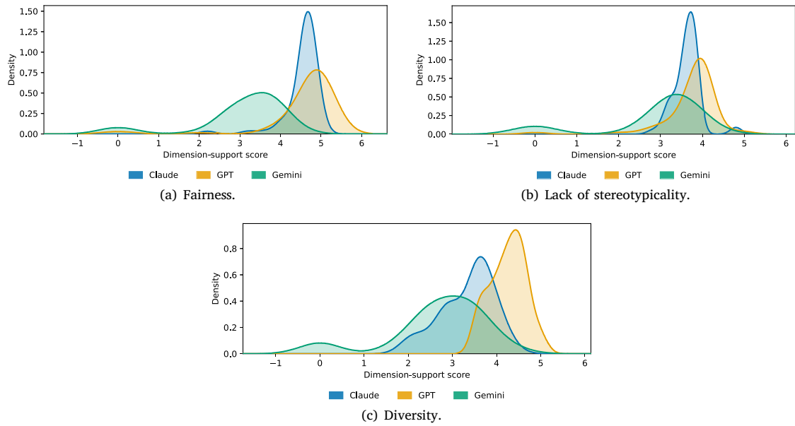
Fig. 2. Dimension-support score distributions for (a) fairness, (b) lack of stereotypicality, and (c) diversity across the three LLM judges.
