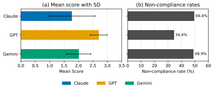
Fig. 3. Set-level dimension-support scores by LLM judge. Error bars represent standard deviations.
