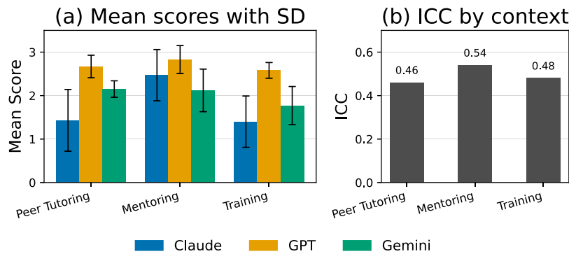
Fig. 7. LLM judge consistency across contexts for persona sets. Error bars represent standard deviations.
