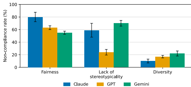
Fig. 5. Non-compliance rates for set-level evaluations across dimensions and LLM judges. Higher values indicate a larger proportion of ratings that did not satisfy the required direct-textual-evidence protocol. Error bars represent standard deviations.
