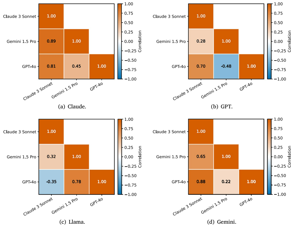
Fig. 4. Pairwise correlations among LLM judge dimension-support scores, shown separately by persona generator.
