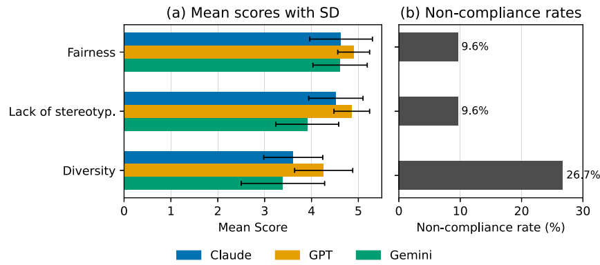
Fig. 1. Individual-level dimension-support scores by LLM judge. Error bars represent standard deviations.
