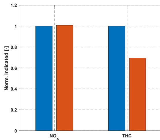
Figure 6. Comparison of indicated emissions ( \text{NO}_x and THC) in simulations and measured, normalized to measurement data.
