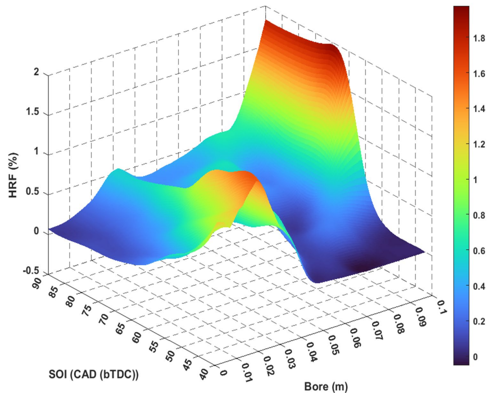
Figure 11. HRF distribution alongside the cylinder radii in various start of injection.
