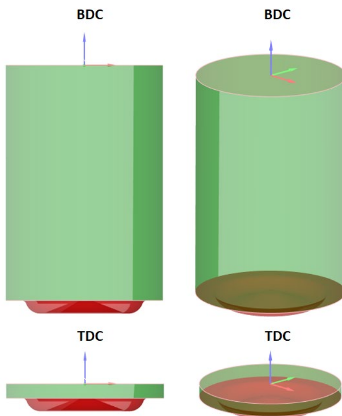
Figure 1. Cylinder closed-loop geometry model positioned at TDC and BDC. XYZ coordinate; x (red), y (green) and z (blue).
