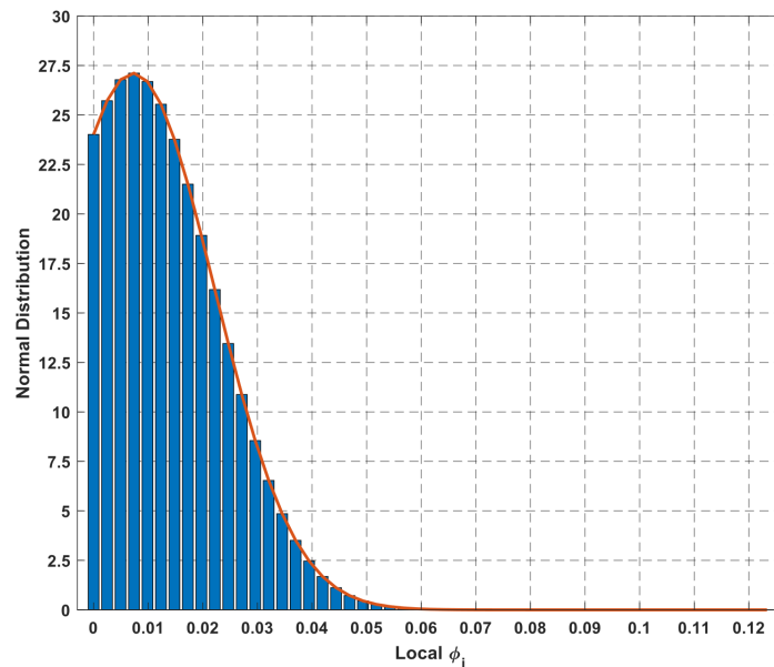
Figure 13. Normal distribution of local equivalence ratio at 16 CAD bTDC for SOI = 66 CAD bTDC.
