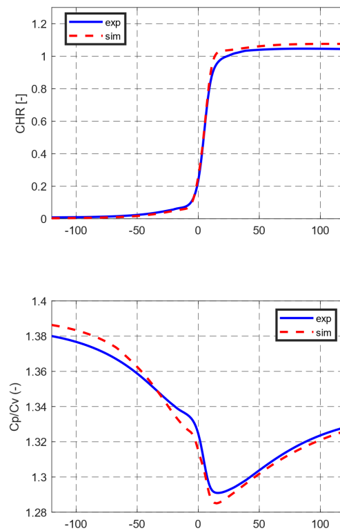
Figure 5. Cumulative heat release and specific heat ratio, compared for experimental and simulation cases.
