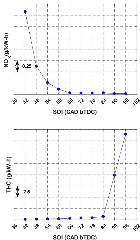
Figure 9. \text{NO}_x and total hydrocarbons (THC) in various selected SOIs.
