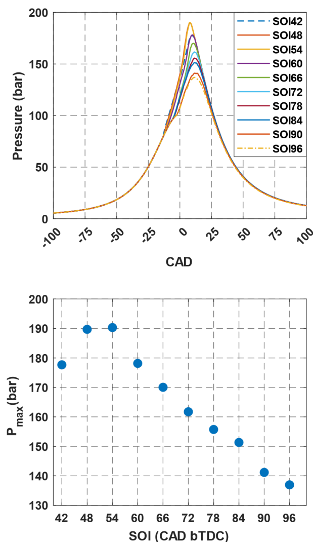
Figure 7. In-cylinder pressure curve and maximum pressure for various injection timing simulations.
