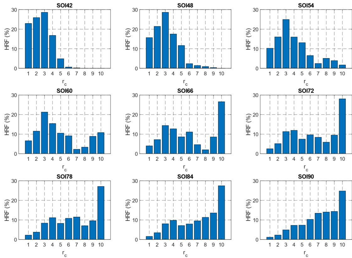
Figure 12. In-cylinder fuel distribution alongside cylinder radii divided to 10 equal zones.
