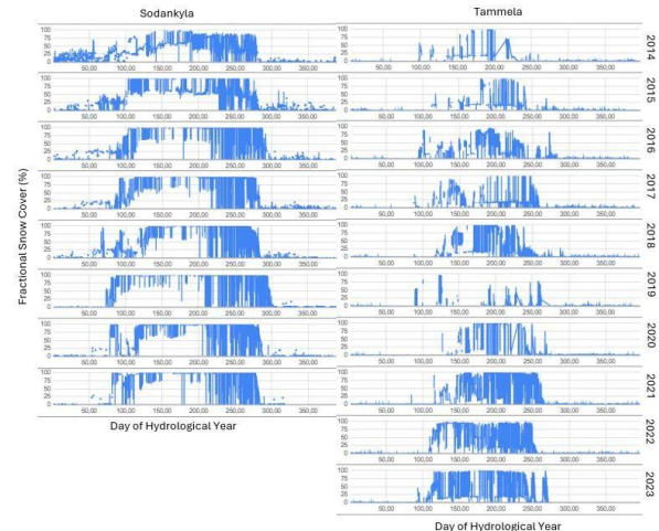
Figure 8. Fractional Snow Cover (%) unvalidated estimations in Tammela and Sodankylä operational monitoring sites during 2014 -2024.
