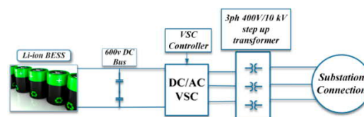
Figure 4. BESS grid integration topology.
