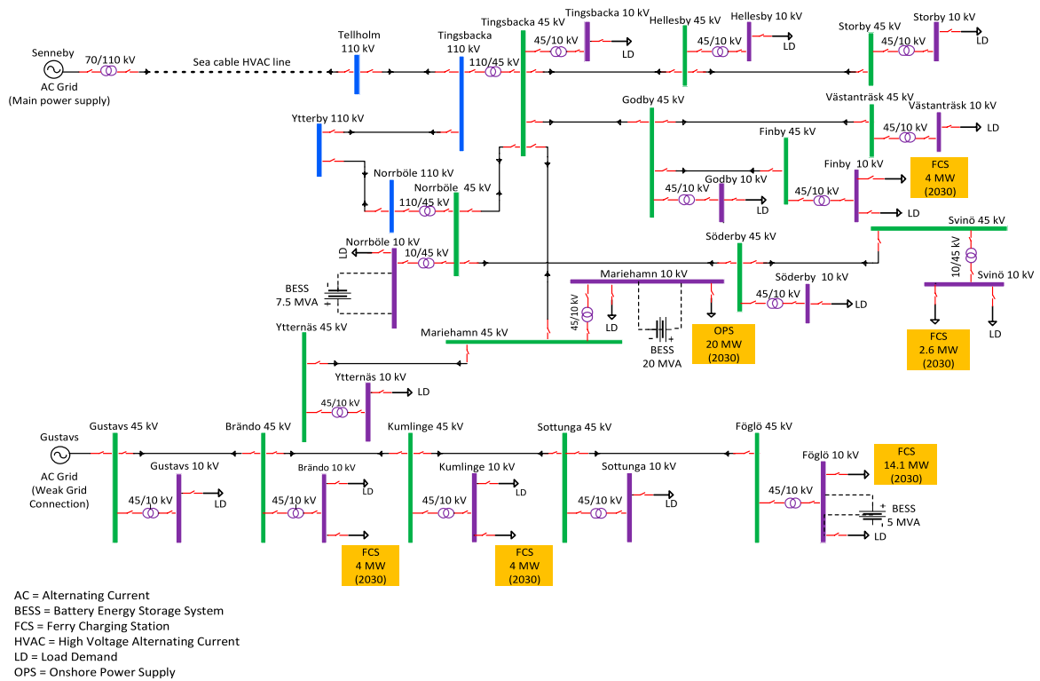
Figure 15. Radial mode operation of the electricity network in the Åland Islands for the year 2030 with BESSs.
