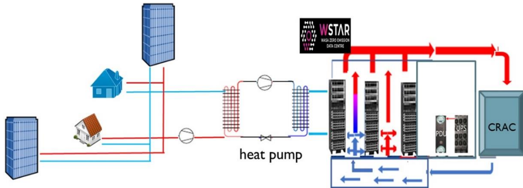
Figure 1 Schematic representation of the DC modeled in this paper.
