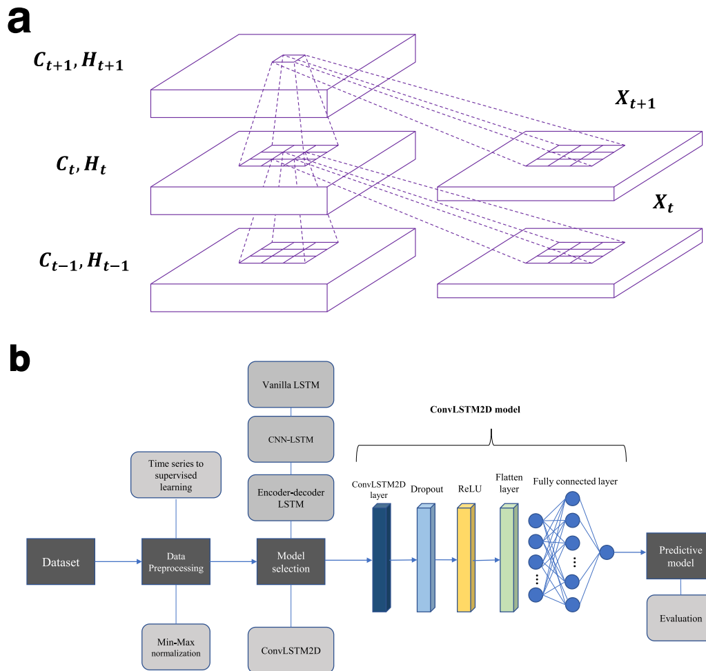
Figure 1. Supervised learning of Bitcoin carbon and energy footprint (a) The ConvLSTM inner structure (Shi et al., 2015) (b) Schematic representation of the model.
