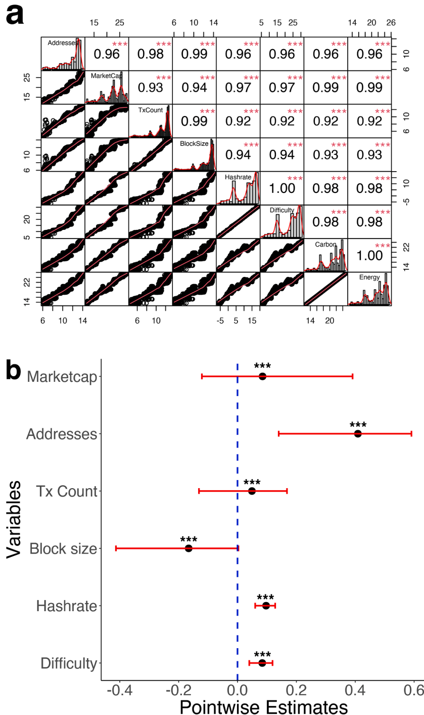
Figure 4. Nexus between BTC carbon footprint, difficulty, hashrate, block size, transaction count, addresses, and market capitalization (a) Statistical analysis using Pearson’s correlation (b) Pointwise estimates using machine learning-based regression technique. Note: *** denotes p -value<0.001, obs # = 4,158, Lambda = 5.2, Tolerance = 0.01, Sigma = 6, Eff. Df = 13.02, R^2 = 0.985 , and Looloss = 195.6.
