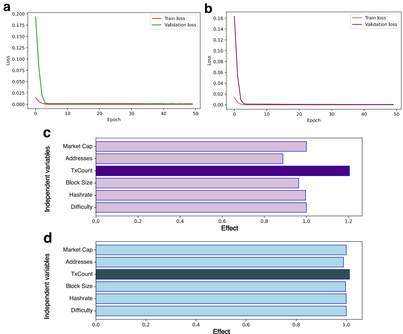
Figure 6. The model training and validation process of ConvLSTM2D model (a) Electricity consumption (b) Carbon emissions. Feature importance of the Prophet's model (c) Electricity consumption (d) Carbon emissions.
