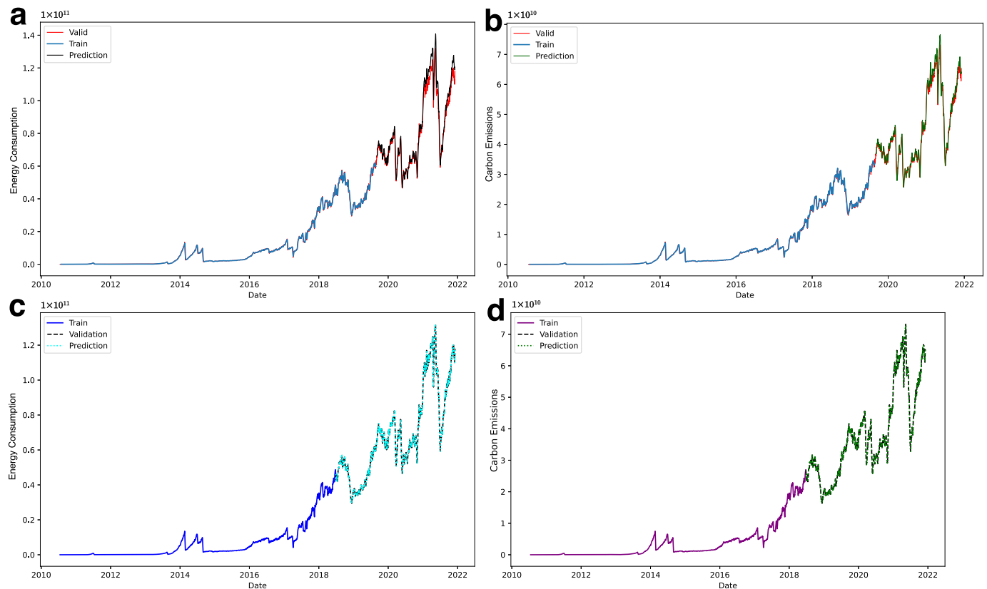
Figure 7. The comparison of ConvLSTM2D model prediction and validation from (a) Electricity consumption (b) Carbon emissions. Comparison of Prophet's model prediction and validation from (c) Electricity consumption (d) Carbon emissions.
