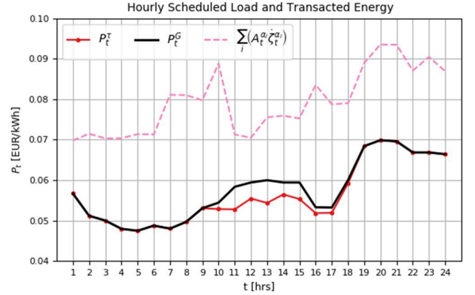
Fig. 4. Hourly energy price paid by reference prosumer (red line), electricity price from the grid (black) and the maximized energy value signal (pink dashed line).
