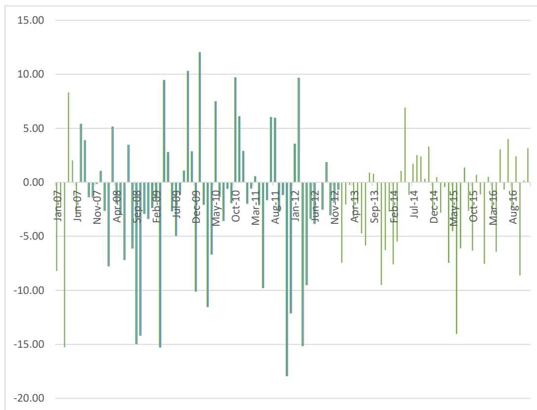
Figure 1: Monthly time-series plot of the 10-1 return spread from January 2007 to January 2017
