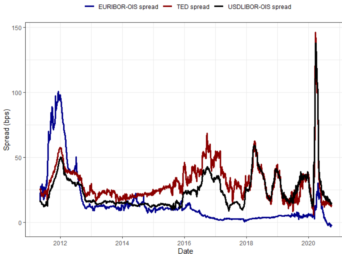
Figure 1. Basis spreads in risk-free rates.
