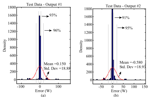
FIGURE 14. The error between targets and output values of ANFIS-FCM model for test sets a) load control b) battery control.
