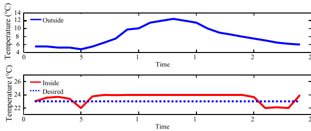
FIGURE 10. Temperature setpoints.
