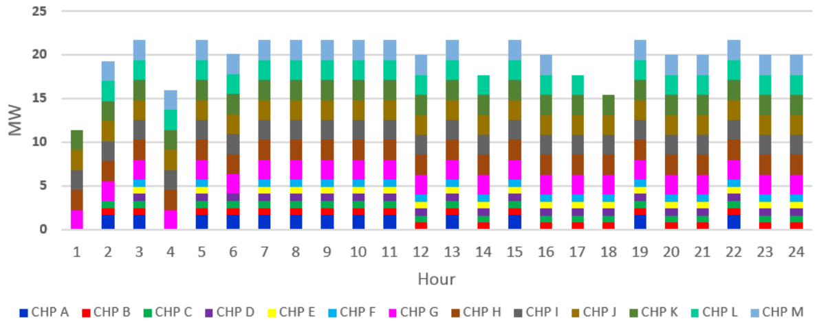
Fig. 12. (a) The CHPs electricity dispatch of the 123-bus system. (b) The CHPs heating dispatch of the 123-bus system.
