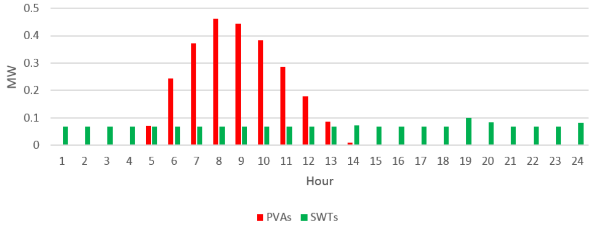
Fig.11. The worst case of the ADS's PVA and SWT electricity generation.
