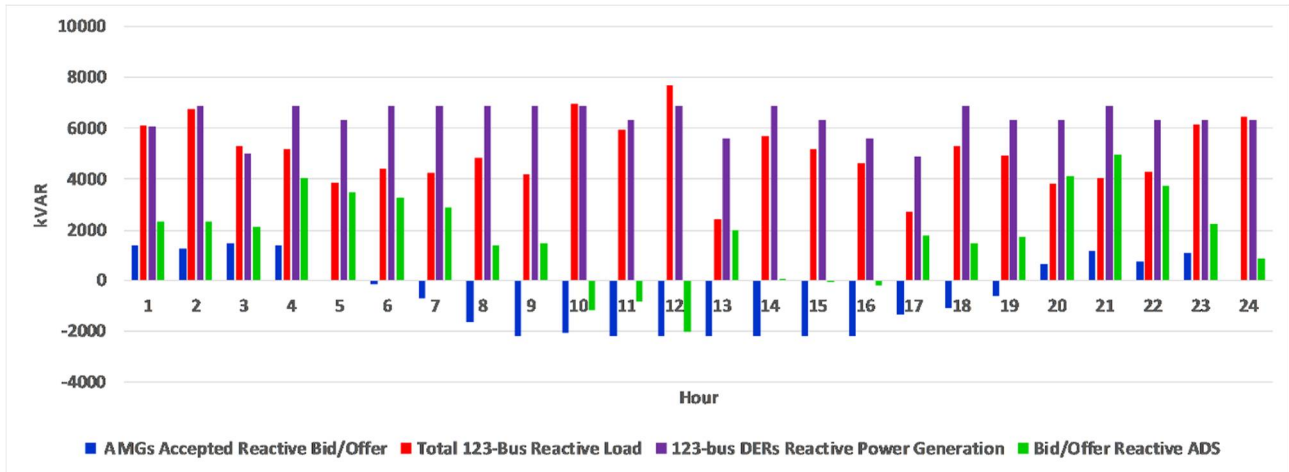
Fig. 18. The aggregated AMGs bid/offer values of reactive power, the 123-bus reactive load, the 123-bus system DERs reactive power generation and the bid/offer values of reactive power of 123-bus system ADS for \beta=1 .
