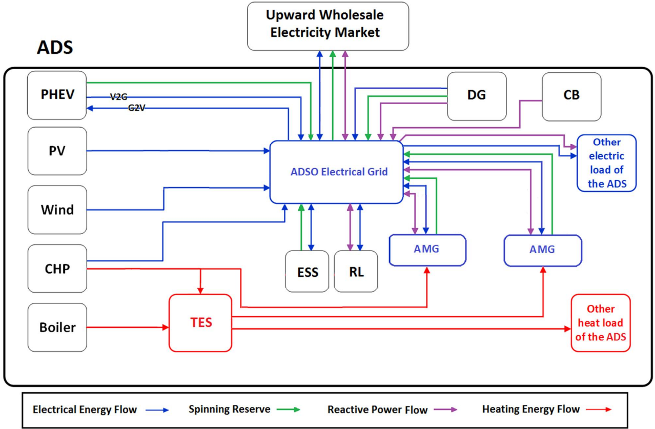
Fig. 2. ADSO energy resources and transactions.
