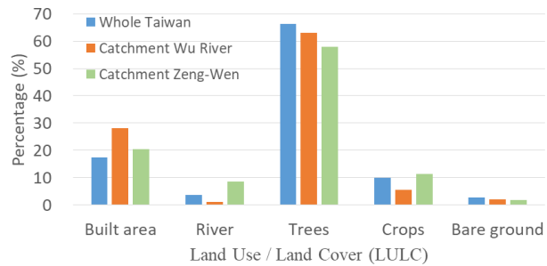
Figure 7. Land Use and Land Cover (LULC) classification and percentages across Taiwan and selected catchments.
