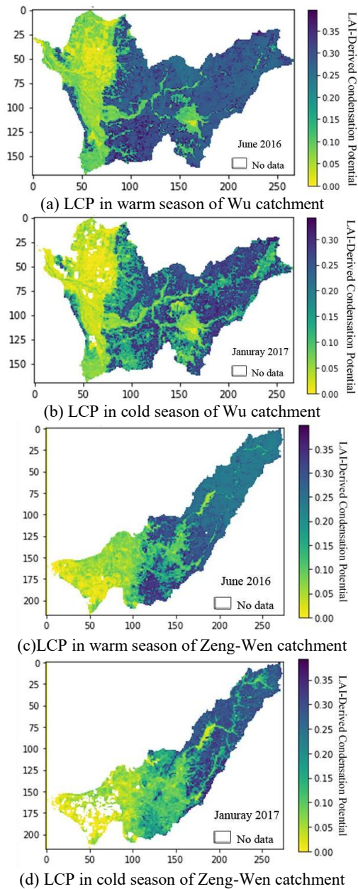
Figure 6. Spatial distribution of the LAI-derived Condensation Potential (LCP) across selected catchments during the warm and cold seasons.
