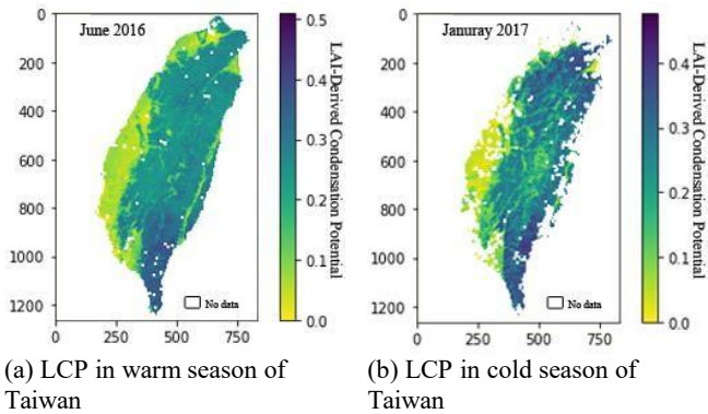
Figure 5. Spatial distribution of the LAI-derived Condensation Potential (LCP) across Taiwan during the warm and cold seasons.
