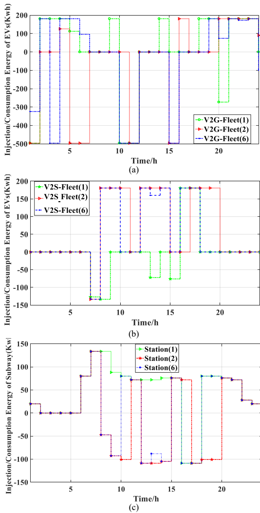
Fig. 11. Energy exchange patterns of fleets 1, 2, 6 for (a) V2G (b) V2S (c) TSPLs energy exchange with grid and EVs
