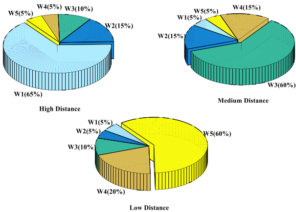
Fig. 9. Probability assignment of each weighting factor in roulette wheel
