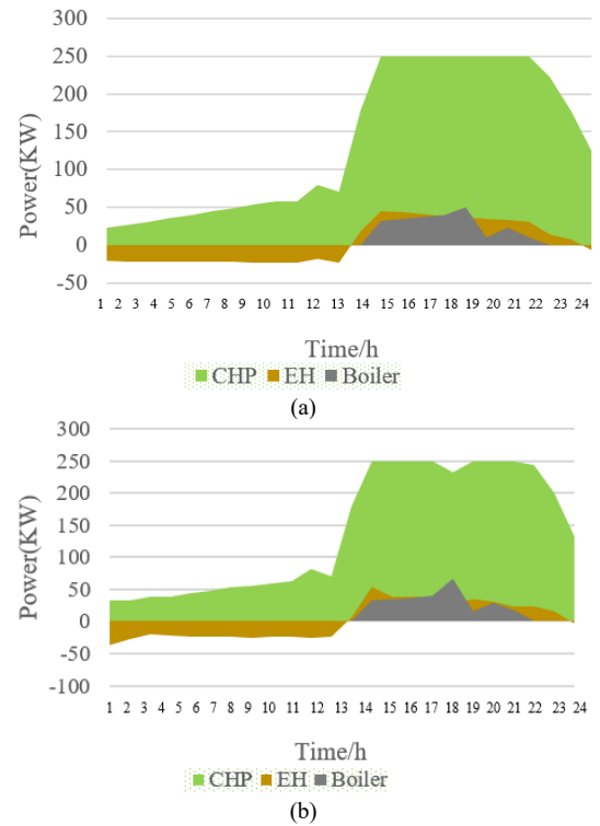
Fig. 13. EH energy trading with the grid a) deterministic b) stochastic
