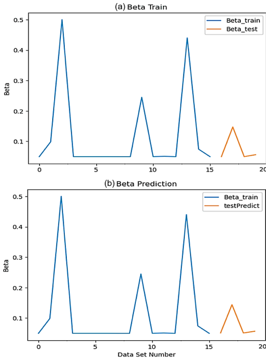
Fig. 5. (a) training and (b) prediction values of \beta for Case A.
