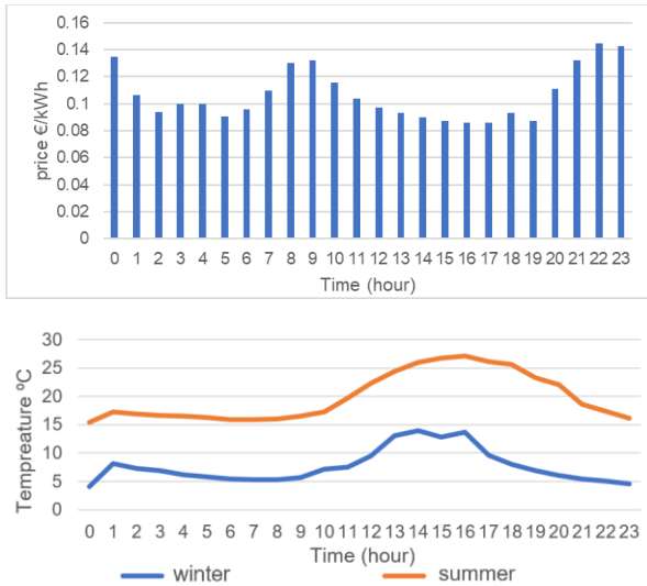
Fig. 3. Hourly electricity price and outdoor temperature.
