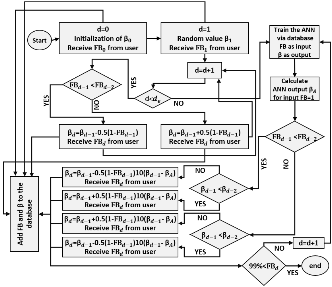
Fig. 2. Flowchart of the proposed ANN-based framework.
