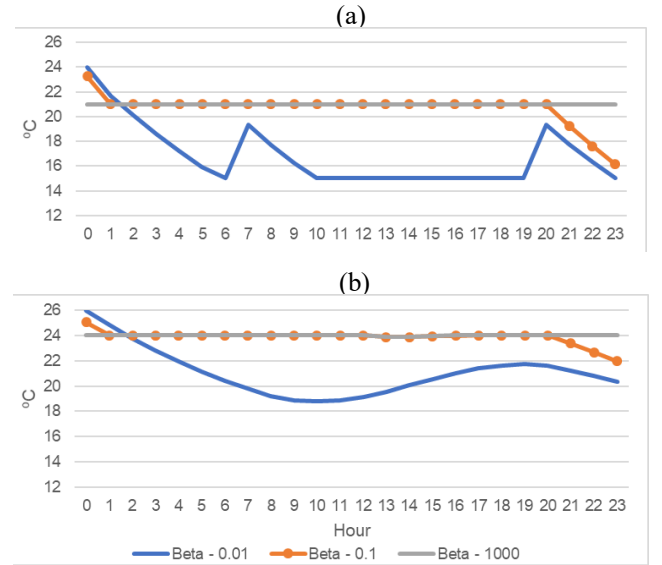
Fig. 4. The indoor temperature in (a) summer and (b) winter.
