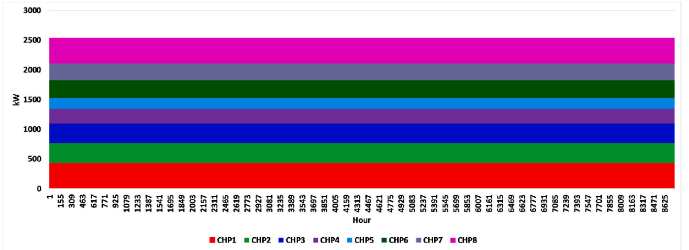
Fig. 15. The electricity generation of combined heat and power generation facilities for the final year of planning and the fourth scenario.
