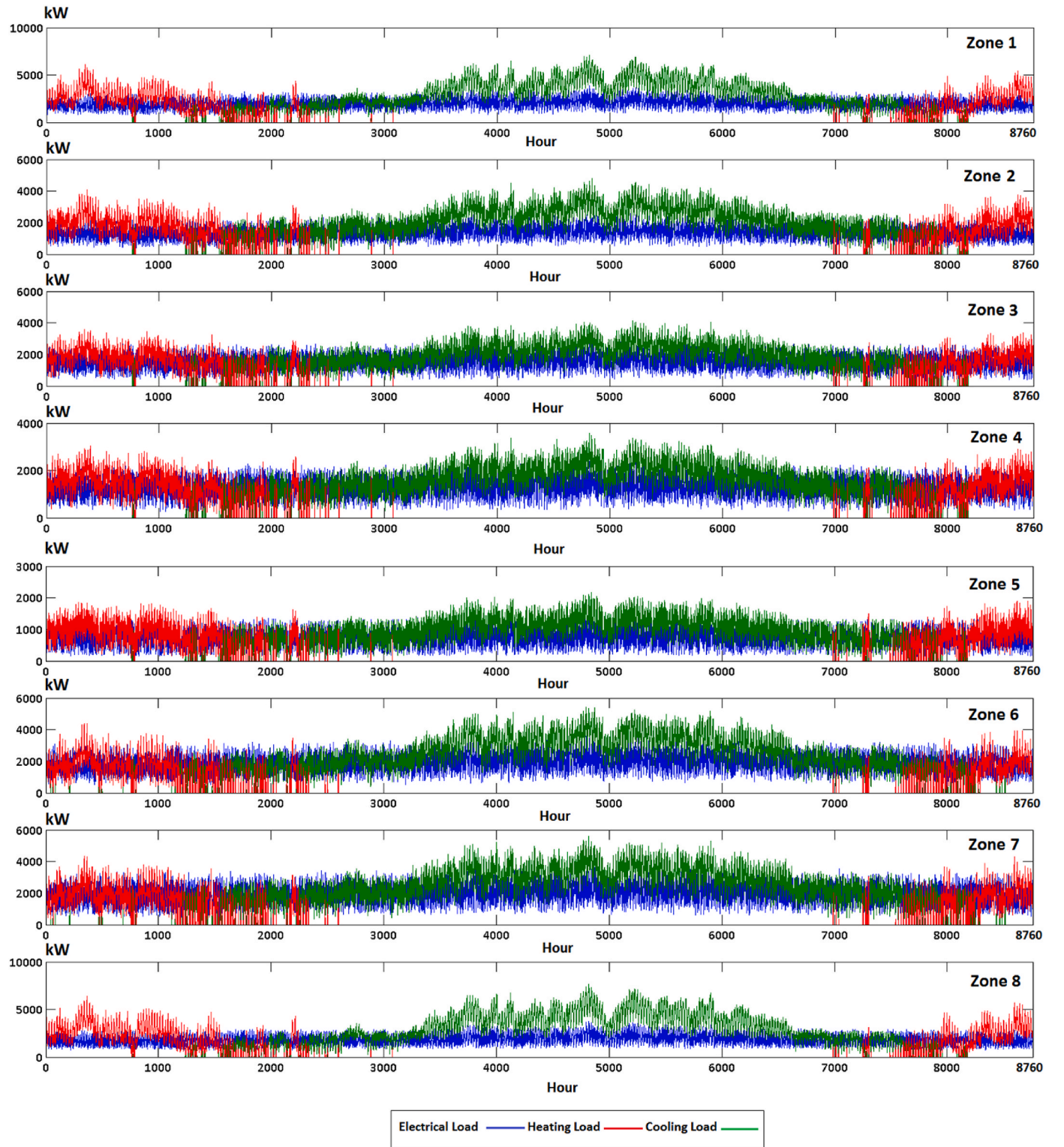
Fig. 3. The estimated values of electrical, heating, and cooling load profiles for the horizon year (2028).
