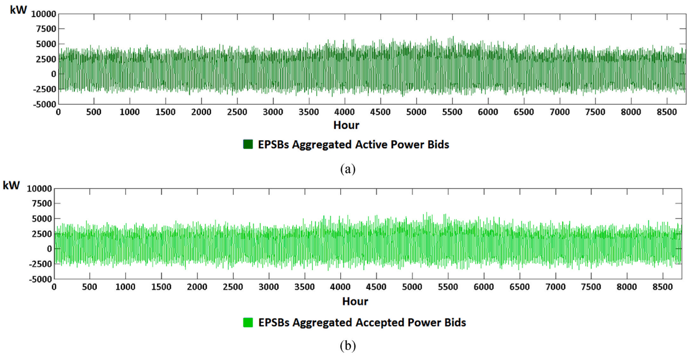
Fig. 12. The submitted values of EPSBs' active power (a), the accepted values of EPSBs' active power (b), the submitted values of EPSBs' reactive power (c), the accepted values of EPSBs' reactive power (d), the submitted values of EPSBs' spinning reserve (e), and the accepted values of EPSBs' spinning reserve (f) of distributed generation for the final year of planning and the fourth scenario.
