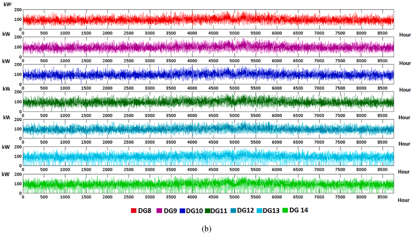
Fig. 13. The estimated values of the active power of 1–7 (a), and 8–14 (b) distributed generation for the final year of planning and the fourth scenario.
