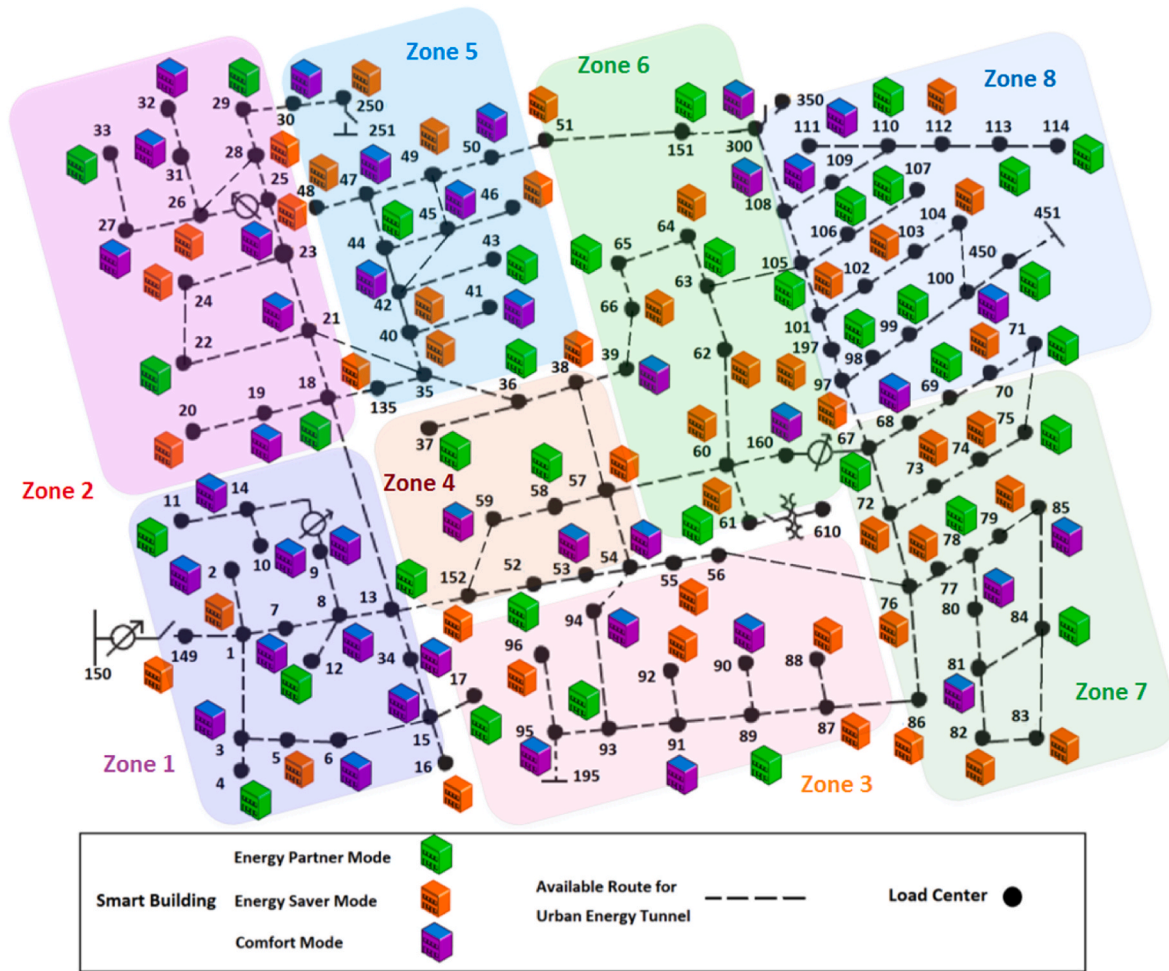
Fig. 2. The modified 123-bus IEEE test system.
