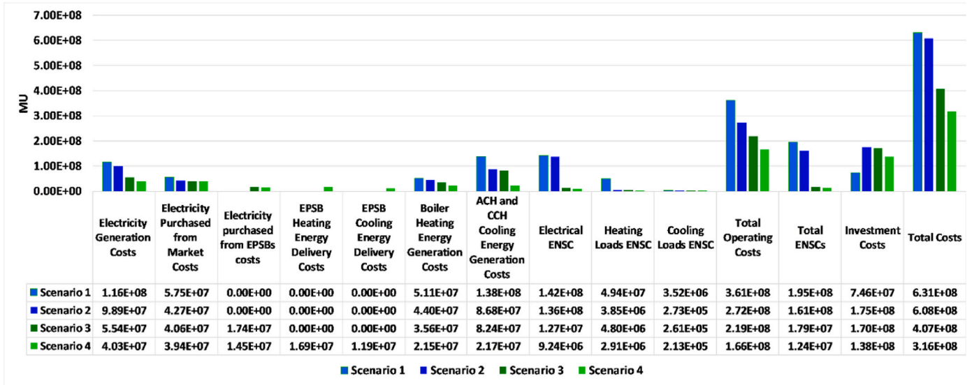
Fig. 21. The final investment costs, energy not supplied costs, electricity generation costs, and operating costs for considered scenarios at the horizon year of planning.
