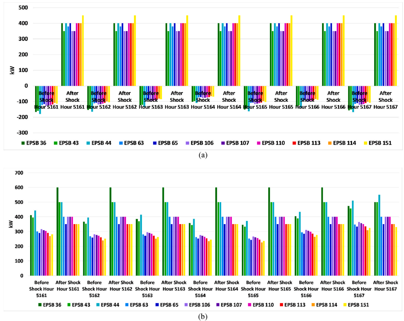
Fig. 25. (a) The energy partner smart buildings electrical energy injection to the system after external shock, (b) The energy partner smart buildings cooling energy injection to the system after external shock.
