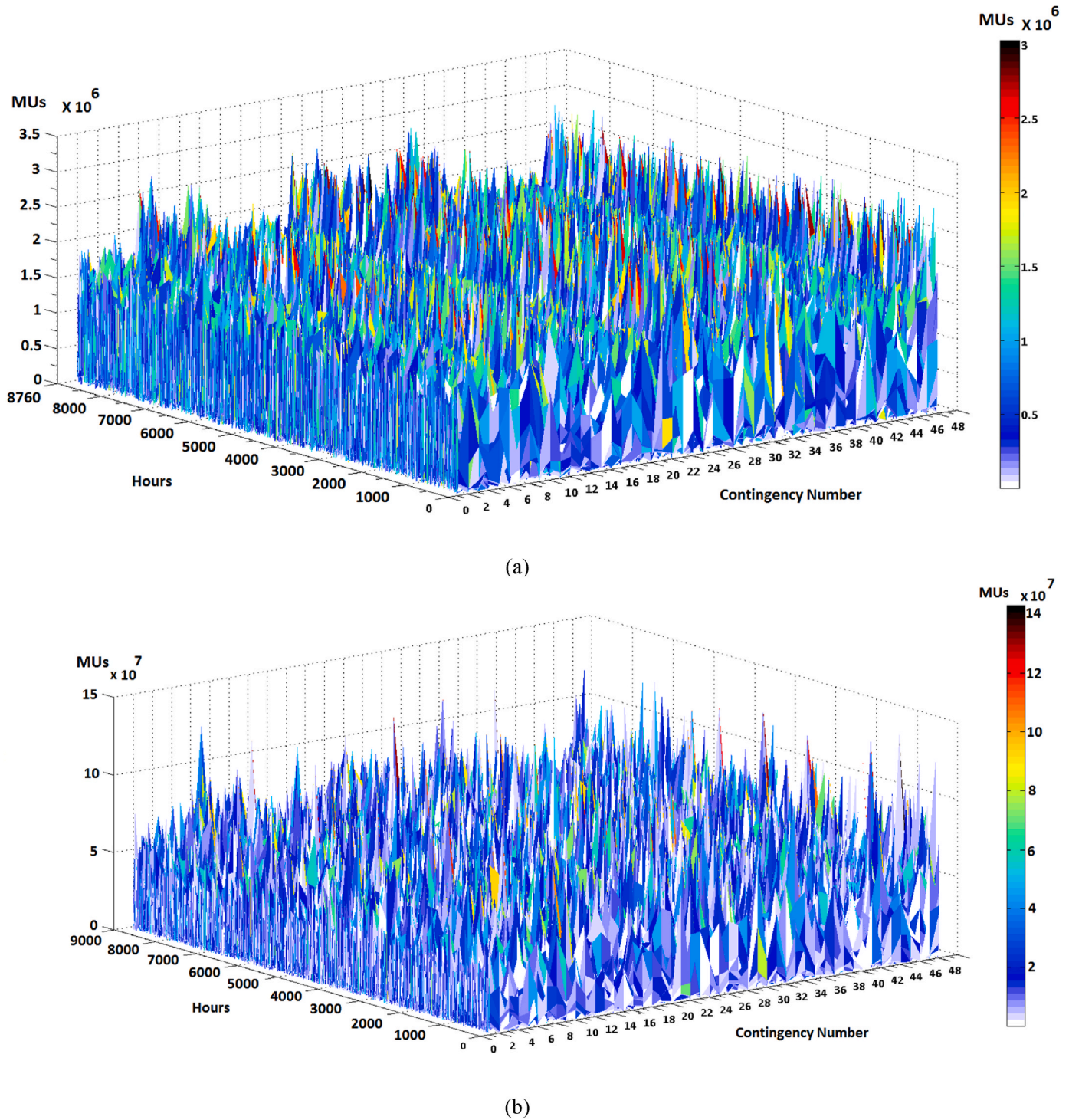
Fig. 19. The aggregated operational and interruption costs of the system for the 48 worst-case external shocks for the fourth (a) and the first scenario (b).
