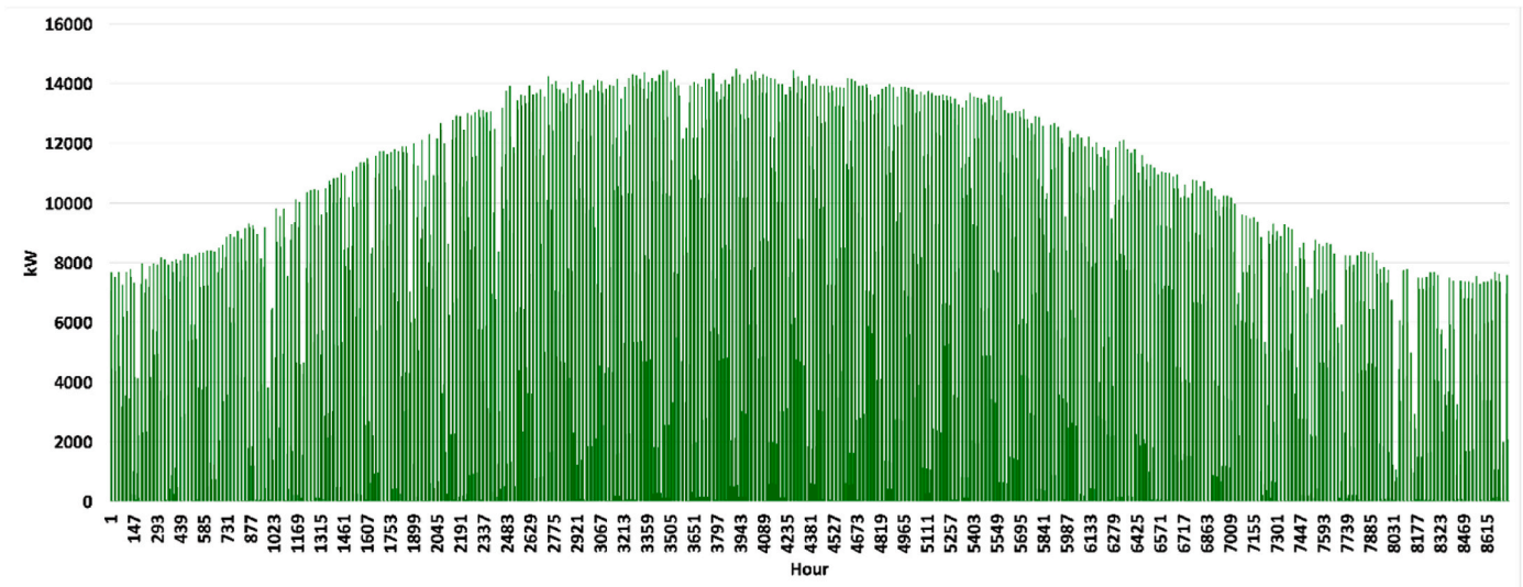
Fig. 5. The forecasted electricity generation of wind turbines for the final year of planning.
