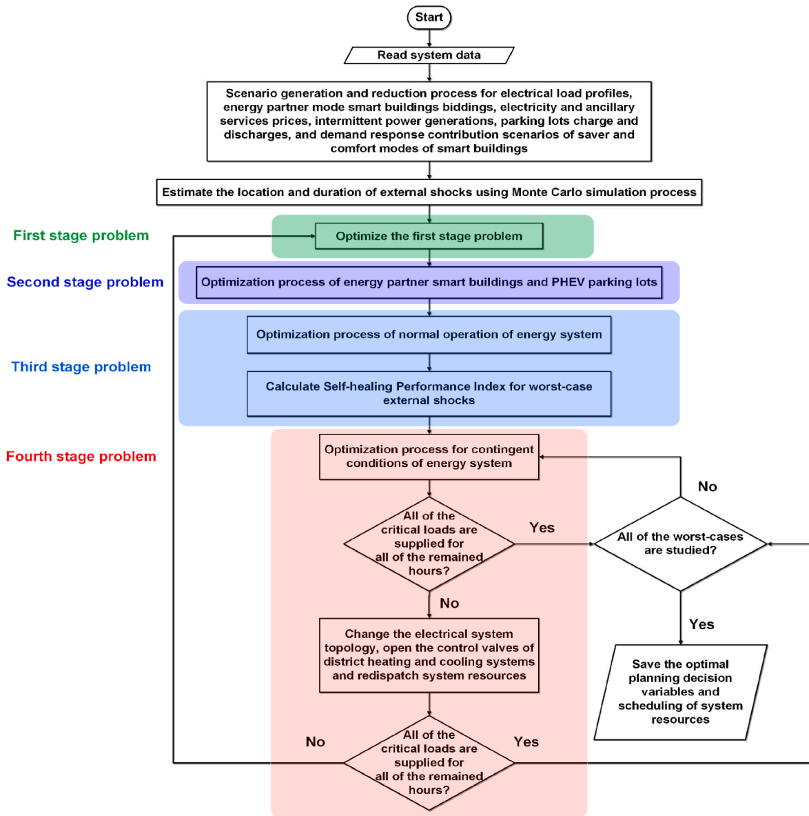
Fig. 1. The overall flowchart of the proposed procedure.
