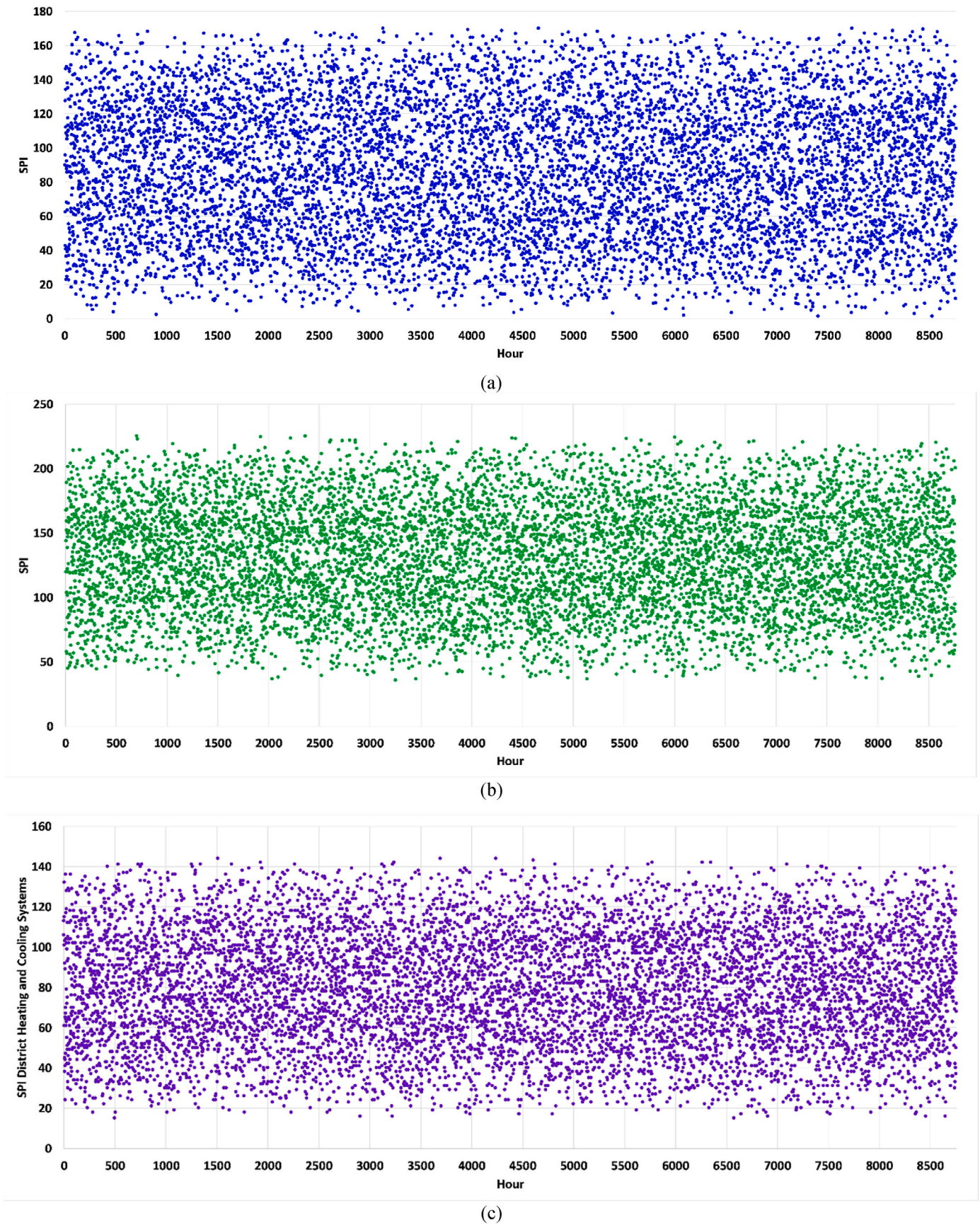
Fig. 20. (a) The self-healing performance index for the designed system of the first scenario and 48 worst-case external shocks. (b) The SPI for the designed system of the second scenario. (c) The SPI for the district heating and cooling designed systems of the third scenario.
