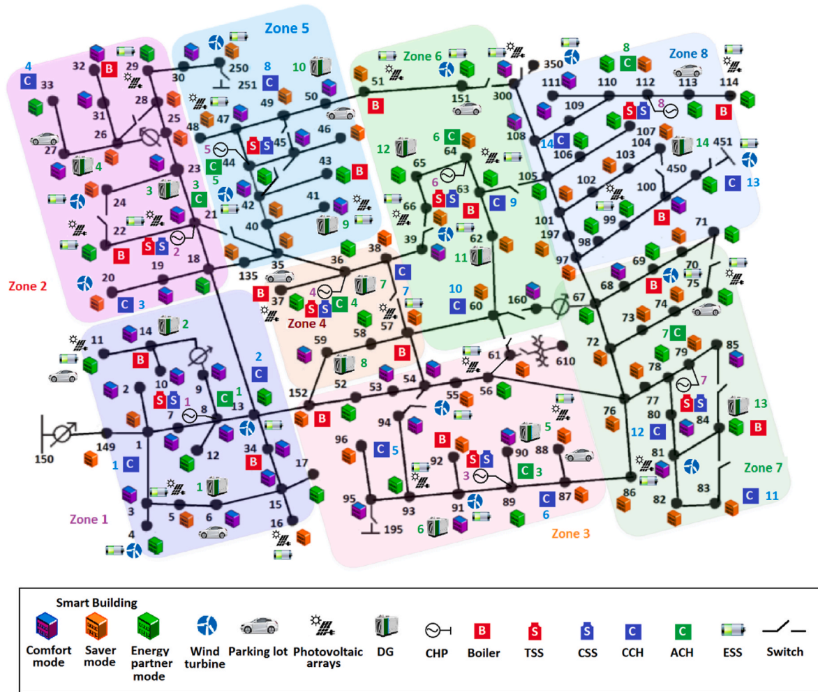
Fig. 6. The optimal topology of the system for the final year of planning and the fourth scenario.
