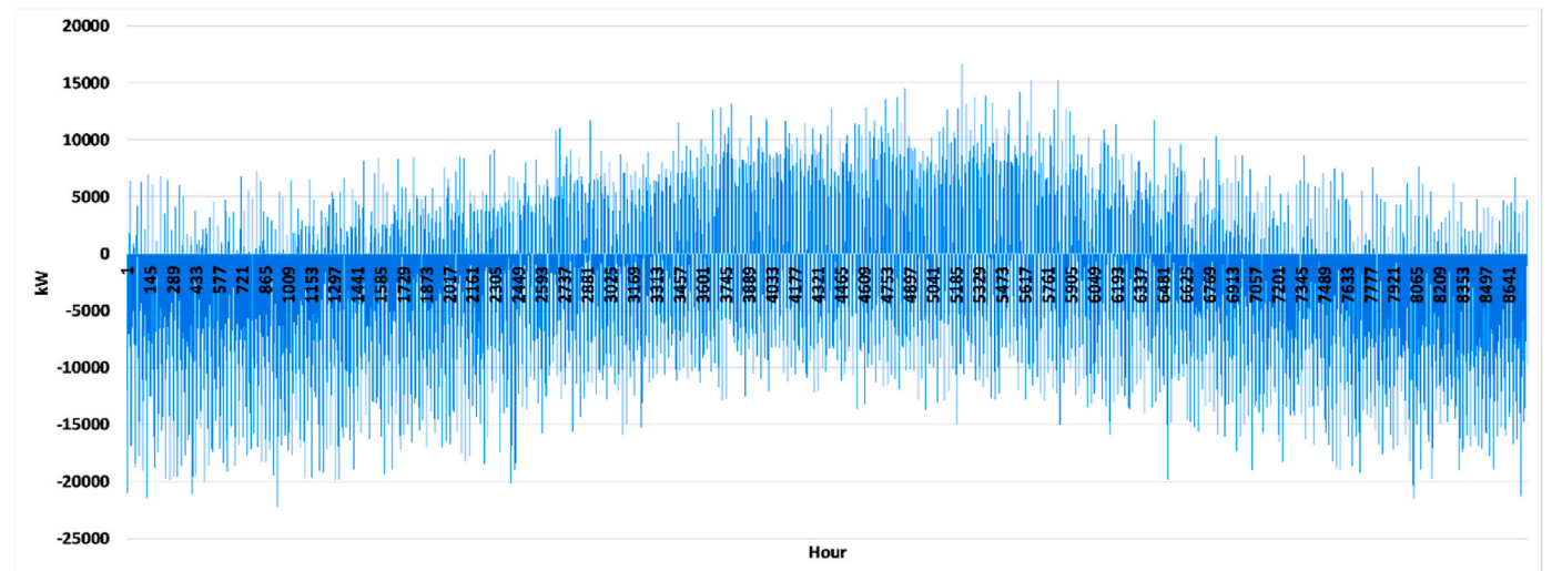
Fig. 18. The electrical energy transactions with the upward electricity market for the final year of planning and the fourth scenario.
