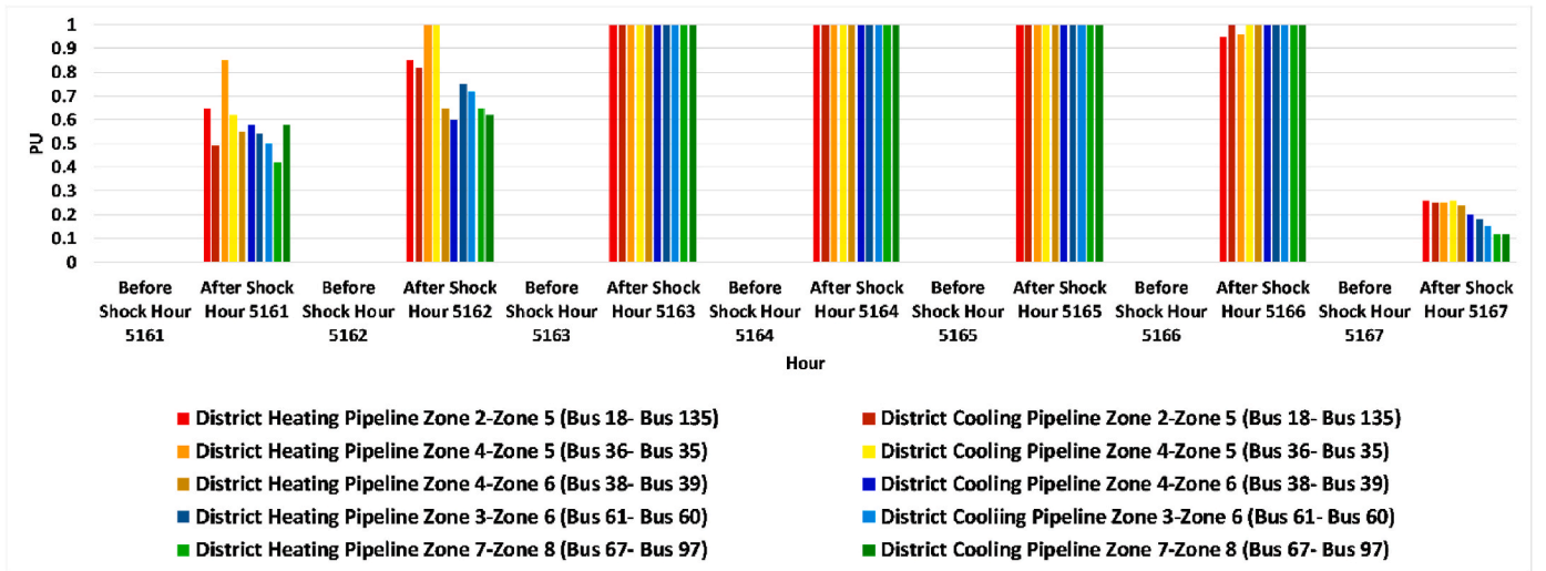
Fig. 23. The heating and cooling energy carriers flow in district heating and cooling pipelines of different zones before and after external shock.
