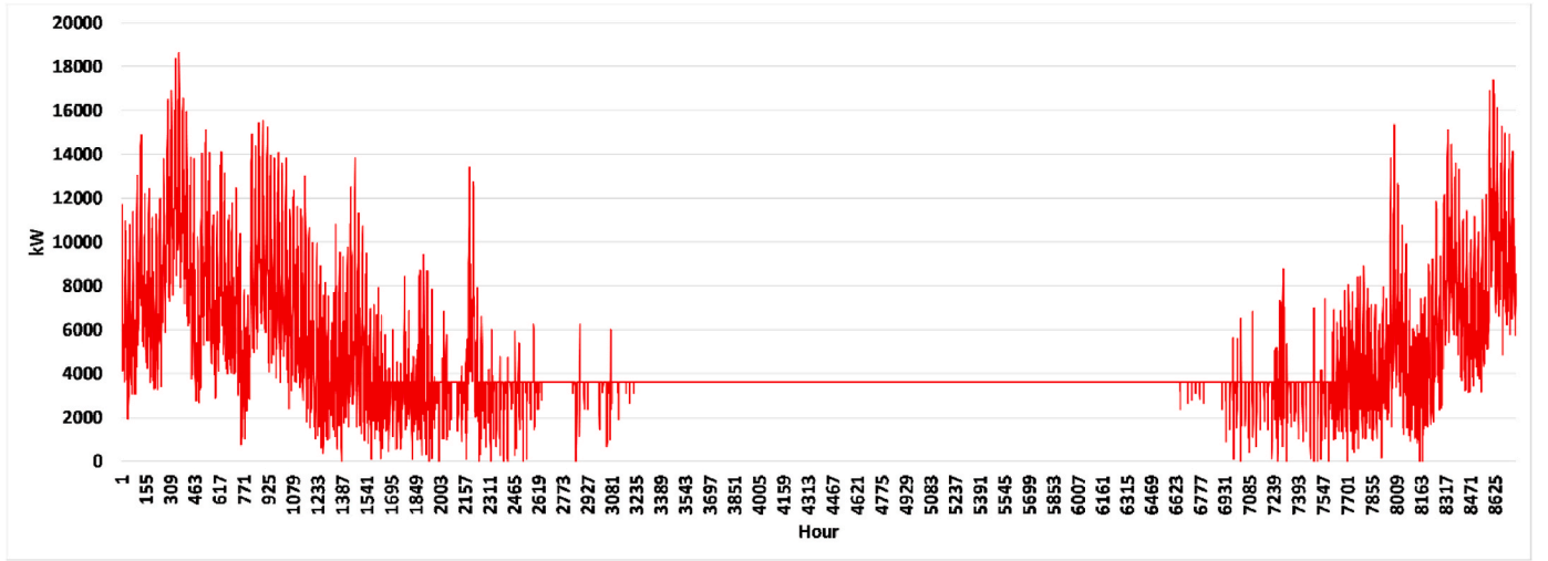
Fig. 14. The estimated values of heating energy generation of boilers for the fourth scenario and the final planning year.
