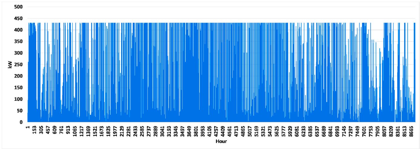
Fig. 4. The forecasted electricity generation of photovoltaic arrays for the final year of planning.
