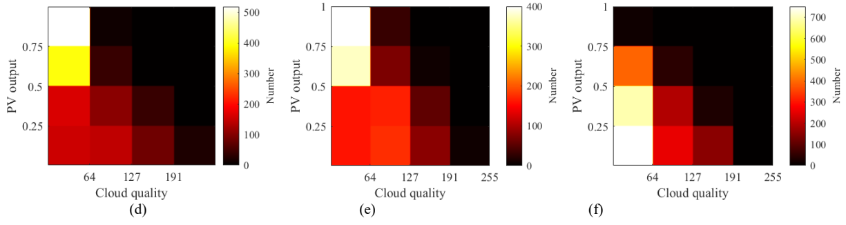
Fig. 5. Relationship between cloud quality values and PV output data. (a)(d) Time horizon ranges from 9:00 to 10:00. (b)(e) Time horizon ranges from 12:00 to 13:00. (c)(f) Time horizon ranges from 16:00 to 17:00.
