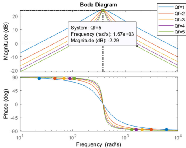
FIGURE 2. Bode diagram of a parallel RLC load with multiples quality factors and resonance frequency at 60 Hz.
