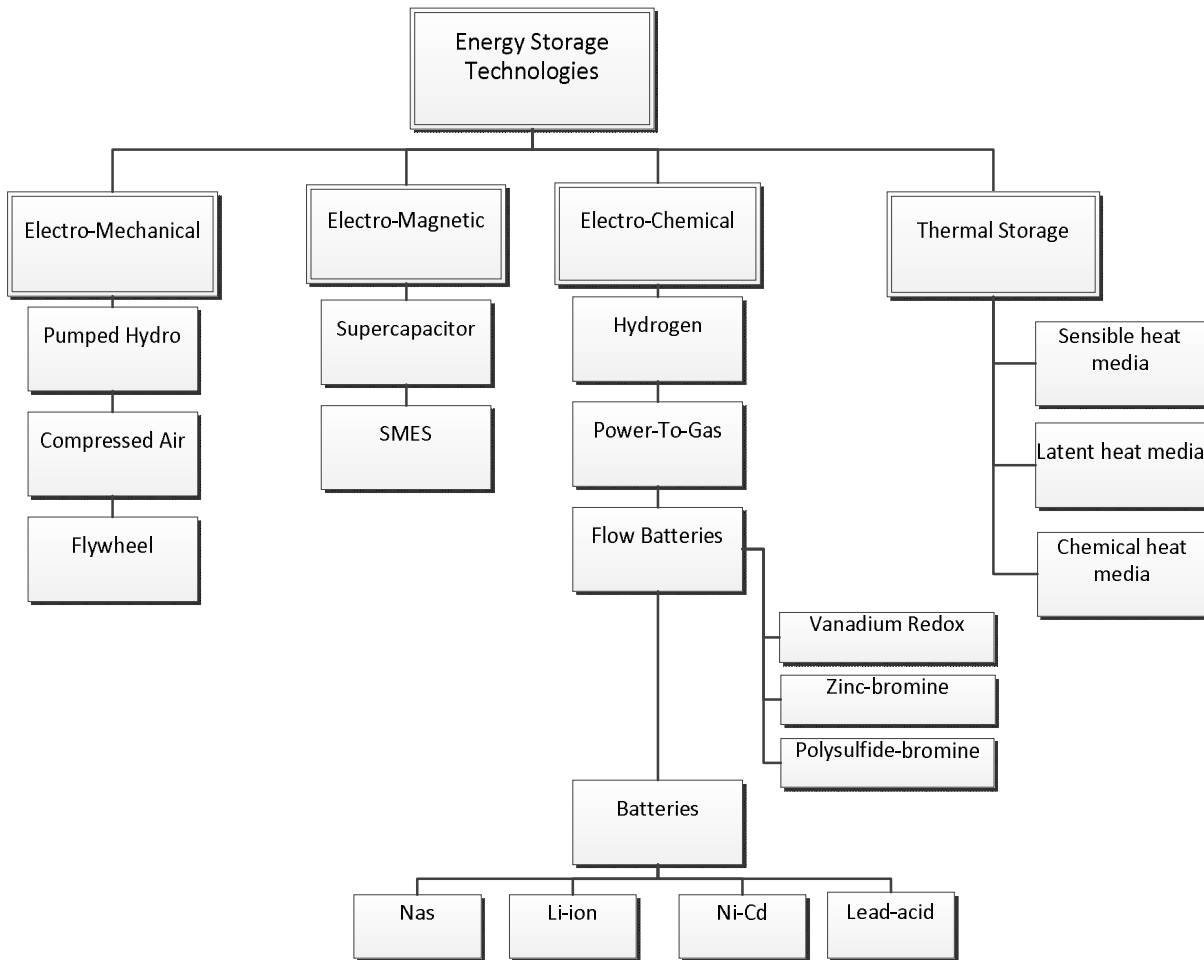
Fig. 5. The main classification of energy storage systems [22]
