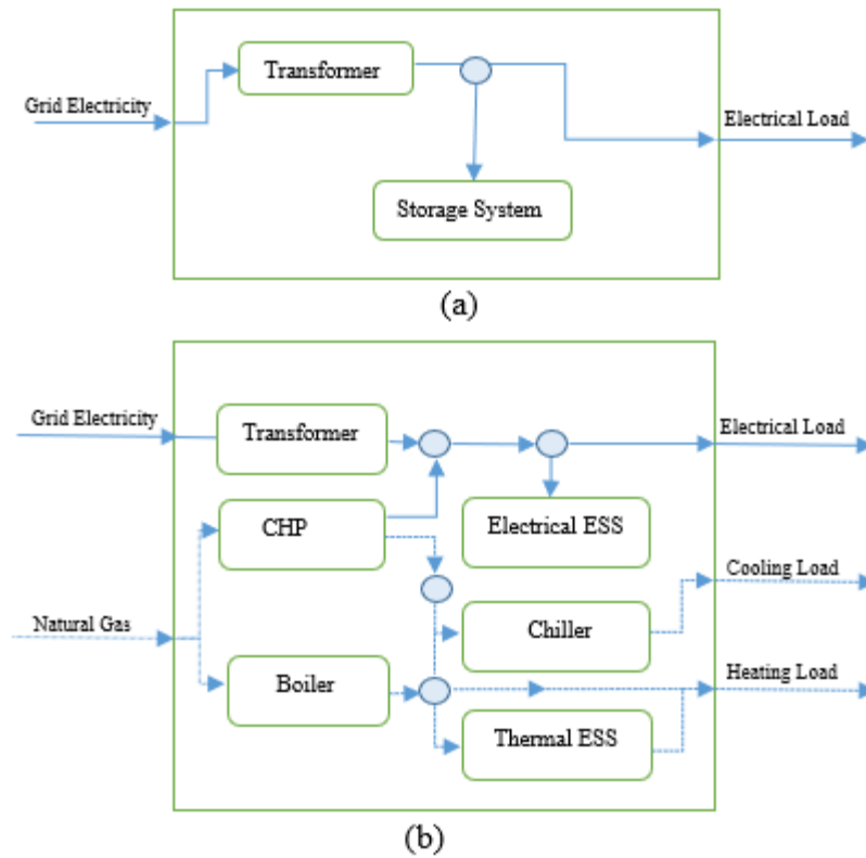
Fig. 8. Multi-energy structure in presence of ESS [42]
