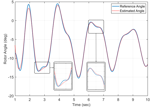
FIGURE 1. Curve-fitting-based estimation of the generator rotor angle.
