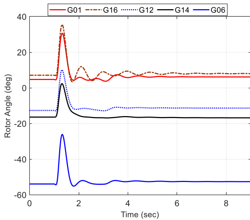
FIGURE 9. Rotor angle oscillations of reference generators (with ward equivalent).
