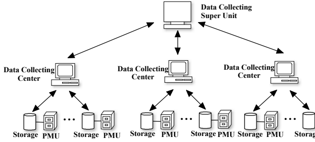
Figure 1. WAMS structure in a smart grid
