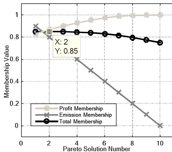
Figure 15: Variation of total membership, profit and emission functions versus Pareto optimal solutions
