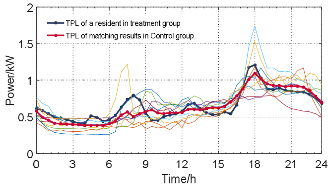
Fig. 7 The performance of pattern matching principle based control objects selection model
