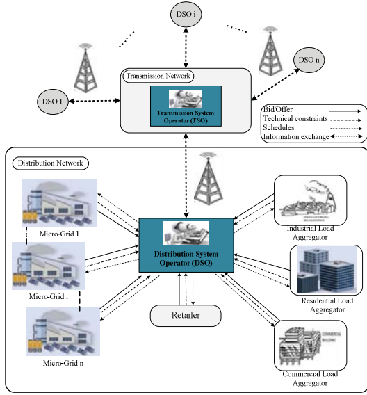
Fig. 1. Proposed structure of local energy market.
