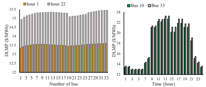
Fig. 5. The amount of DLMP in base case
