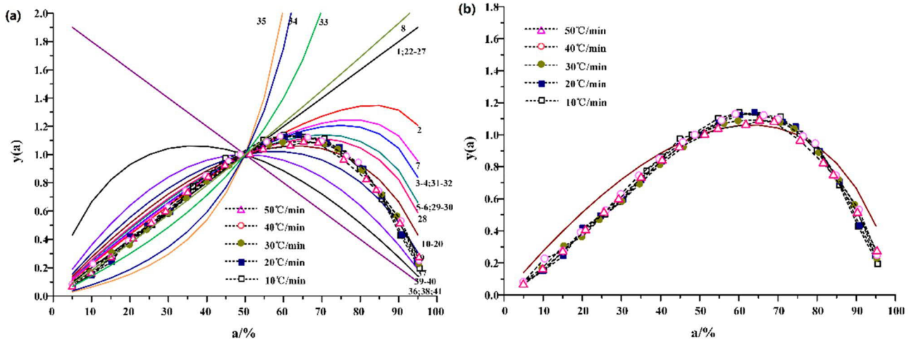
Figure 2. Standard and experimental curves of y(\alpha) - \alpha under N_2 .
