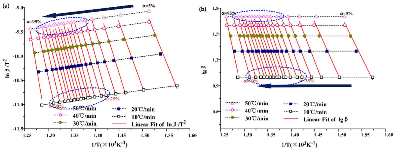
Figure 5. Calculating curve of activation energy under N_2 .
