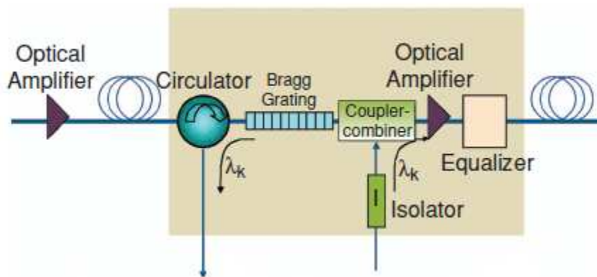
Figure 15. Optical Add/Drop Multiplexing based on Fiber-Bragg Grating (Kartalopoulos 2002)
