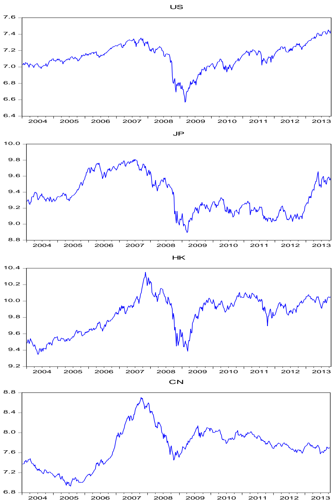
Figure 4. Time series of the indexes (local currency: natural logarithm of the index).
