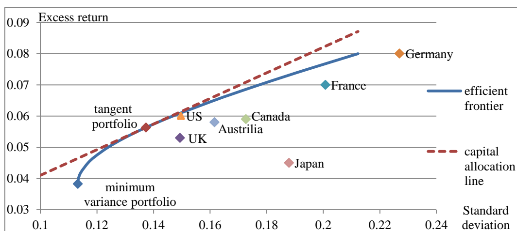
Figure 2. International portfolio diversification. (Source: Bodie et al. 2009: 231–236).
