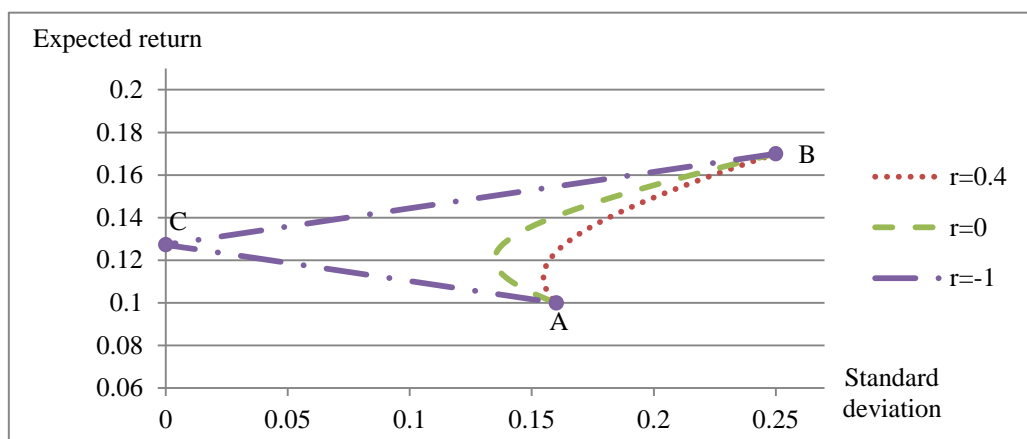
Figure 1. Possible combinations of expected return and standard deviation formed with assets A and B. (Source: Bodie et al. 2009: 201–203).
