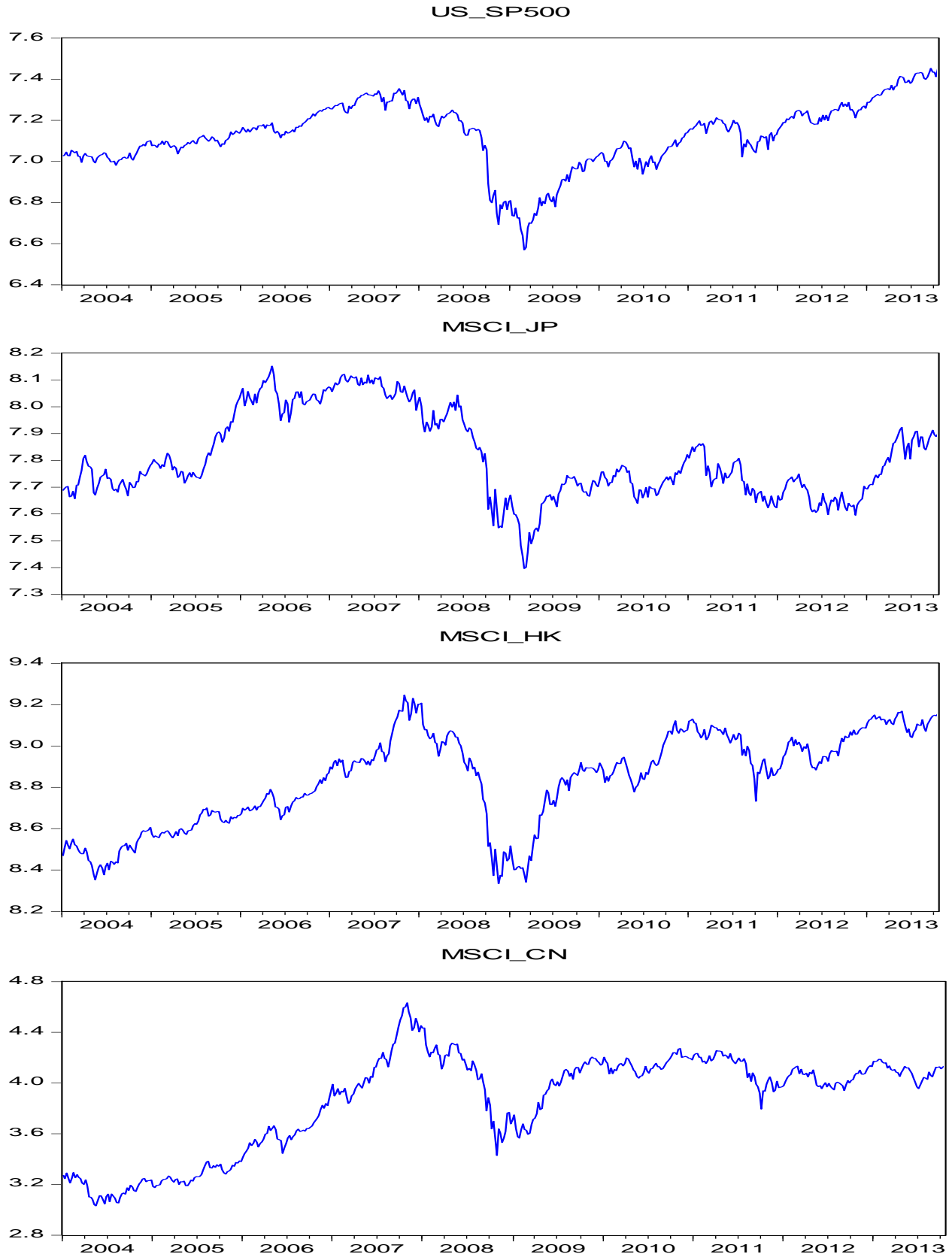
Figure 5. Time series of the indexes (common currency: natural logarithm of the index).
