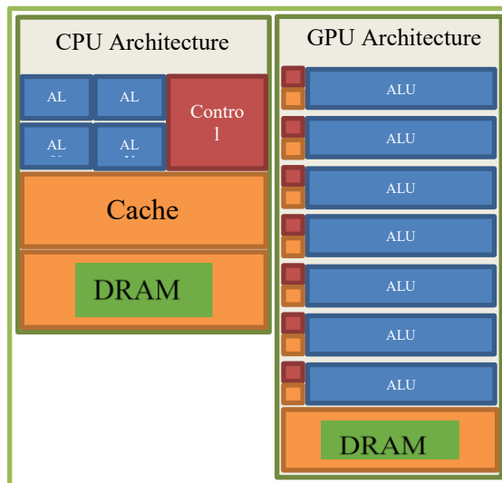
Fig. 2. The Architecture of the CPU and GPU.
